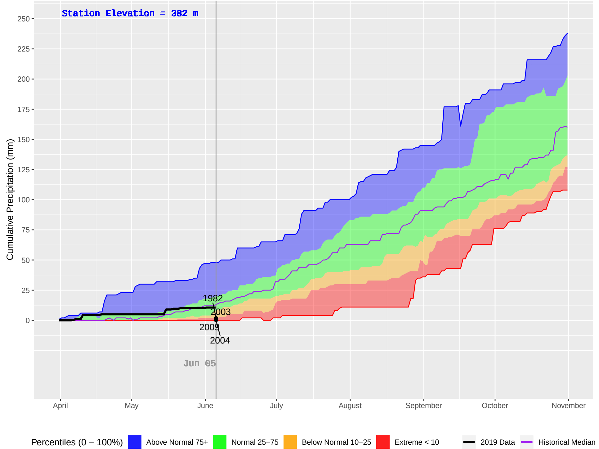
TELEGRAPH CREEK (110) : Historical (1978–2018), Current (2019) Daily Cumulative Precipitation
