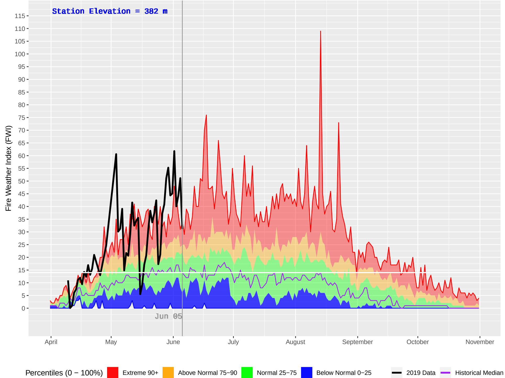
TELEGRAPH CREEK (110) : Historical (1978–2018) and Current (2019) Daily Fire Weather Index (FWI)
