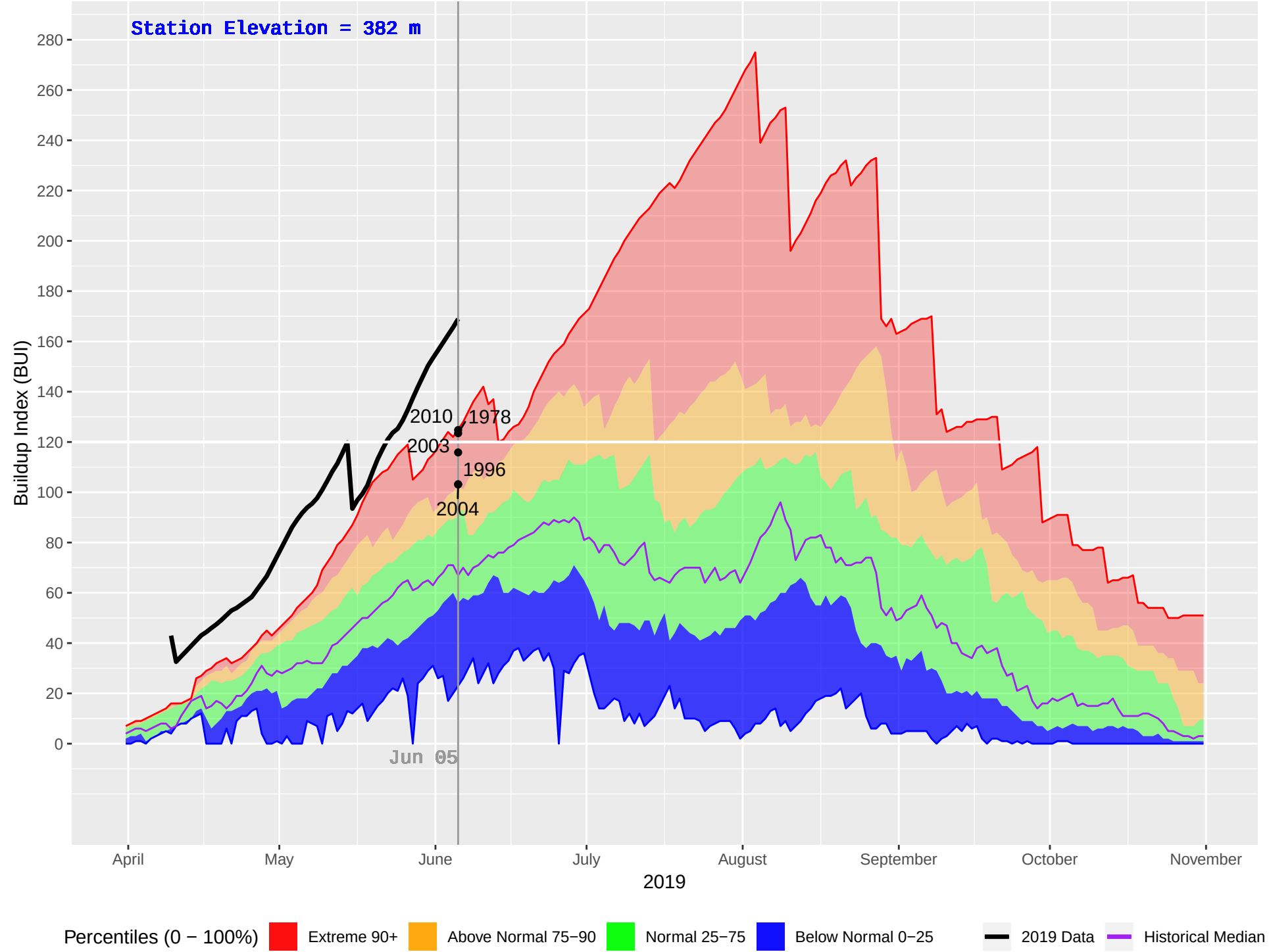
TELEGRAPH CREEK (110) : Historical (1978–2018), Current (2019) Daily Buildup Index (BUI)
