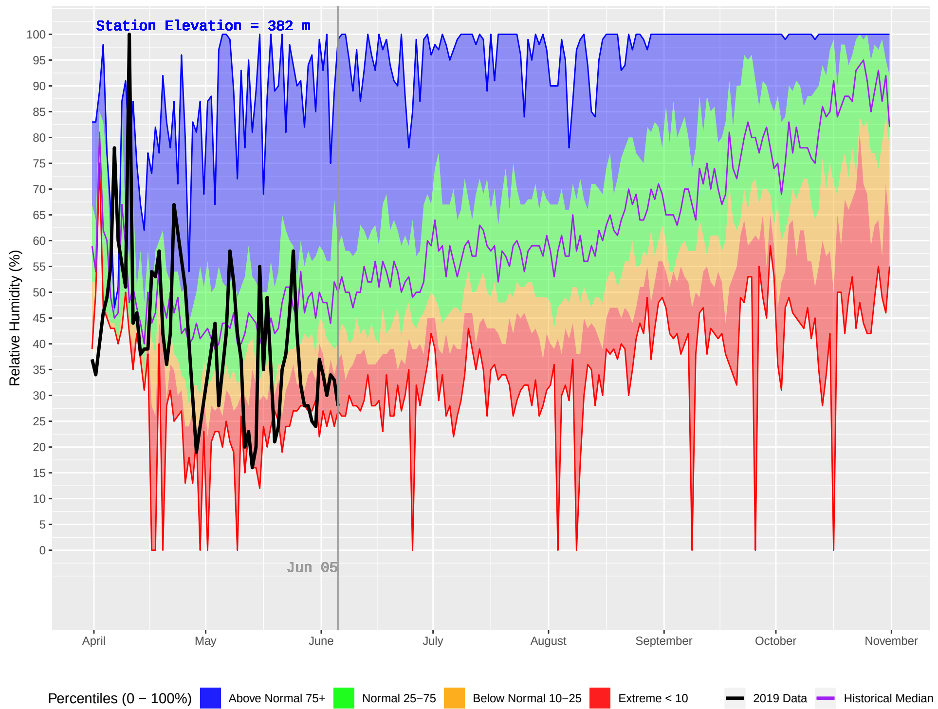
TELEGRAPH CREEK (110) : Historical (1978–2018) and Current (2019) Daily Relative Humidity
