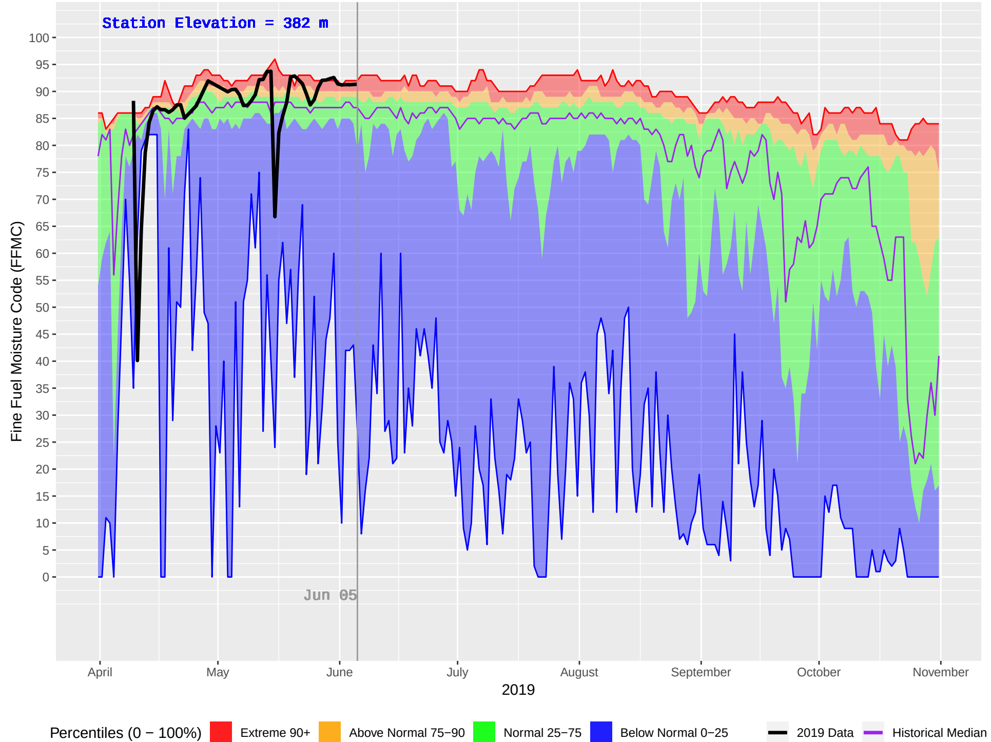
TELEGRAPH CREEK (110) : Historical (1978–2018) and Current (2019) Daily Fine Fuel Moisture Code (FFMC)
