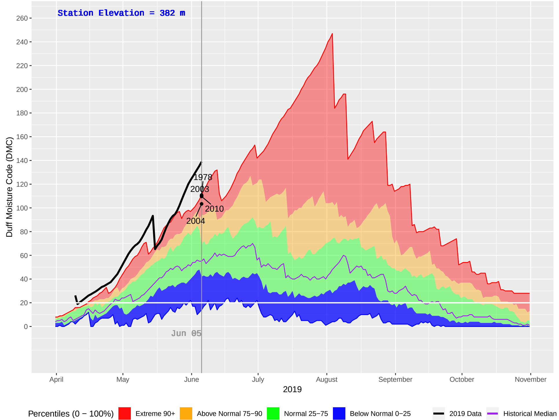
TELEGRAPH CREEK (110) : Historical (1978–2018), Current (2019) Daily Duff Moisture Code (DMC)
